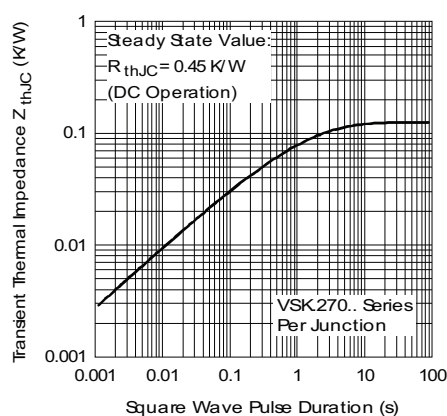
Fig. 22 - Thermal Impedance Z_{thJC} Characteristics
