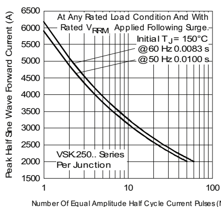
Fig. 8 - Maximum Non-Repetitive Surge Current
