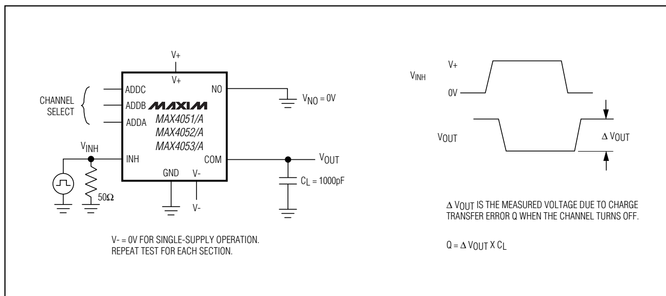
Figure 5. Charge Injection
