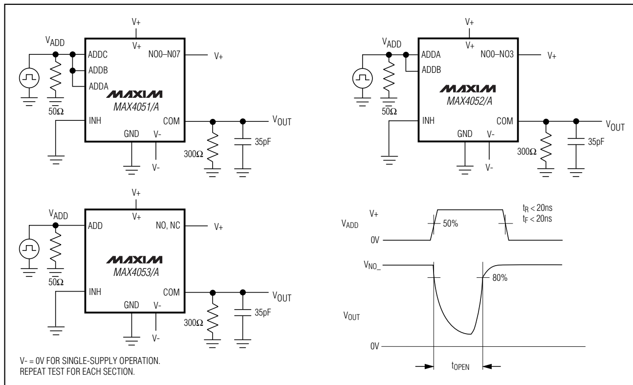
Figure 4. Break-Before-Make Interval
