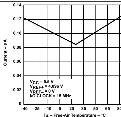
Figure 20. External Reference Current vs Free-air Temperature
