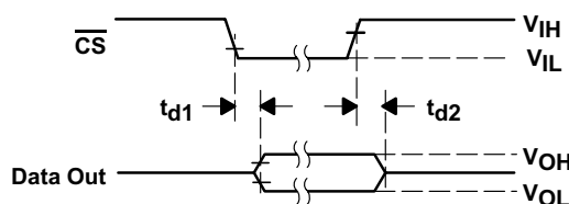
Figure 31. DATA OUT to Hi-Z Voltage Waveforms
