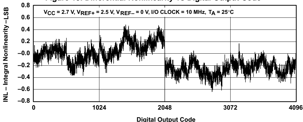
Figure 16. Integral Nonlinearity vs Digital Output Code
