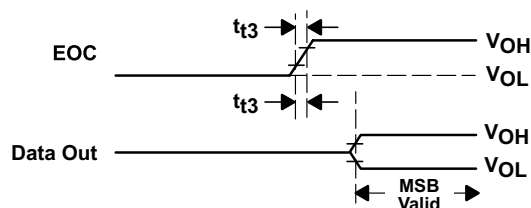
Figure 36. EOC and DATA OUT Voltage Waveforms
