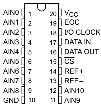
Pin Functions
