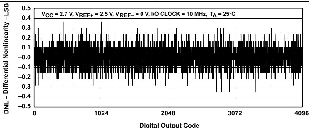
Figure 15. Differential Nonlinearity vs Digital Output Code
