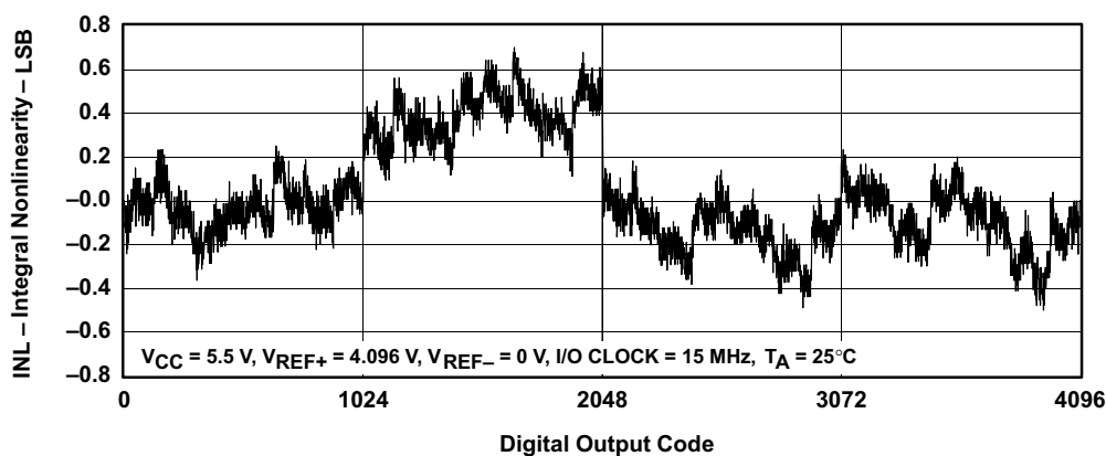
Figure 28. Integral Nonlinearity vs Digital Output Code
