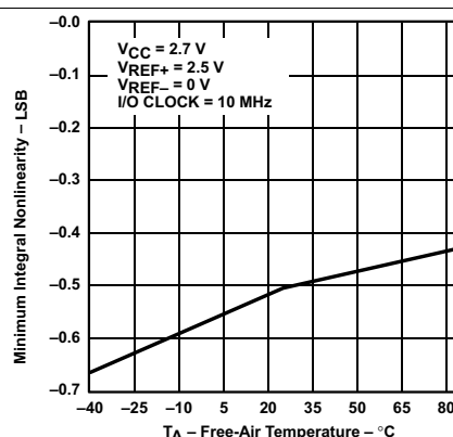
Figure 14. Minimum Integral Nonlinearity vs Free-air Temperature
