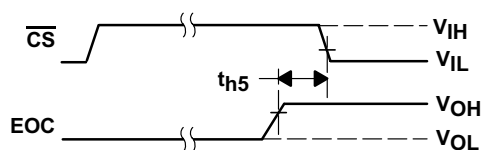
Figure 37. \overline{\text{CS}} and EOC Waveforms
