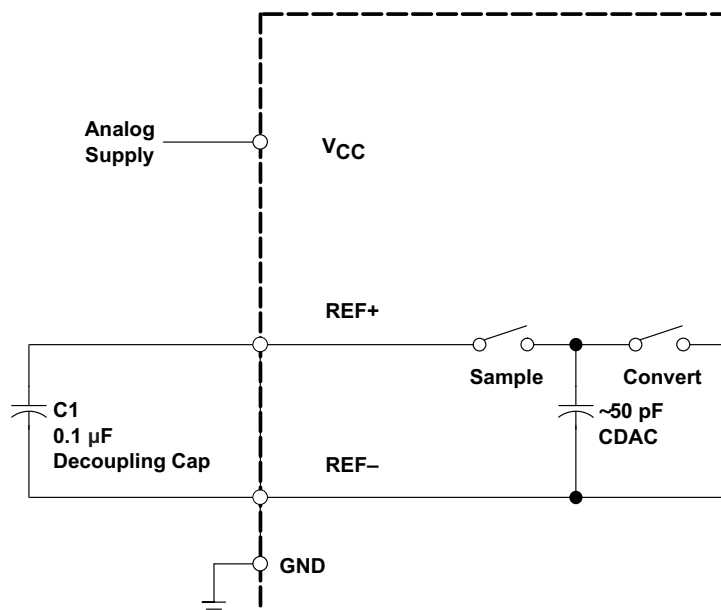
Figure 39. Reference Block Diagram
