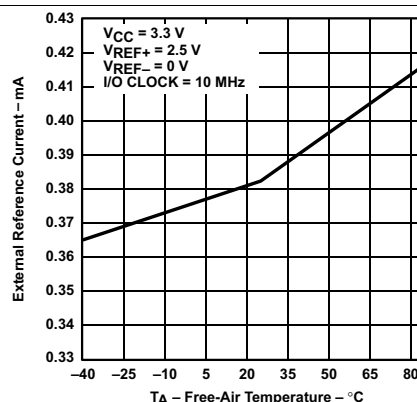
Figure 8. External Reference Current vs Free-air Temperature
