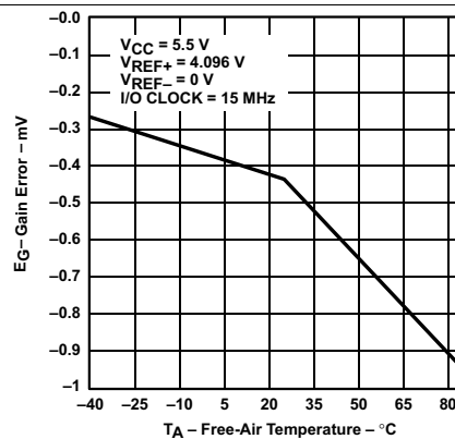
Figure 30. Gain Error vs Free-air Temperature
