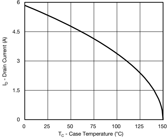
Current Derating*
