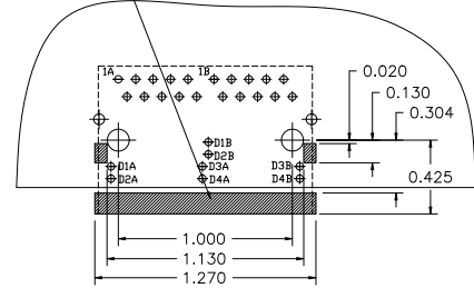
SUGGESTED PCB KEEP OUT AREA (Component Side)
