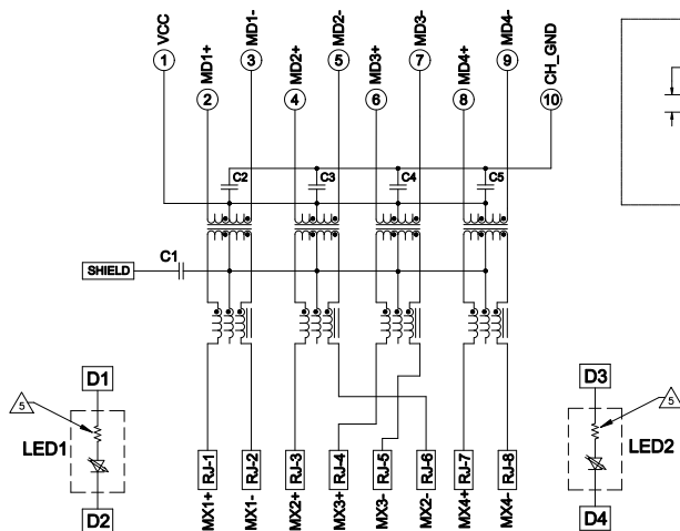
PIN DESIGNATIONS
