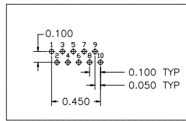
PIN DESIGNATIONS
