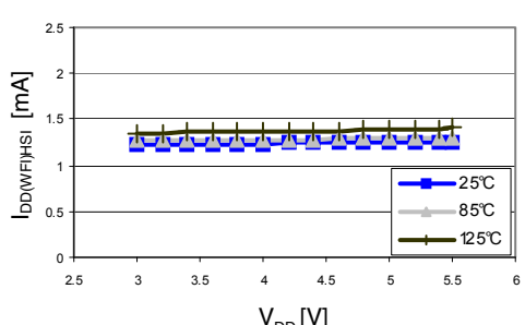
Figure 18. Typ. I_{DD(WFI)HSI} vs. V_{DD} @ f_{CPU} = 16 MHz, peripherals = off
