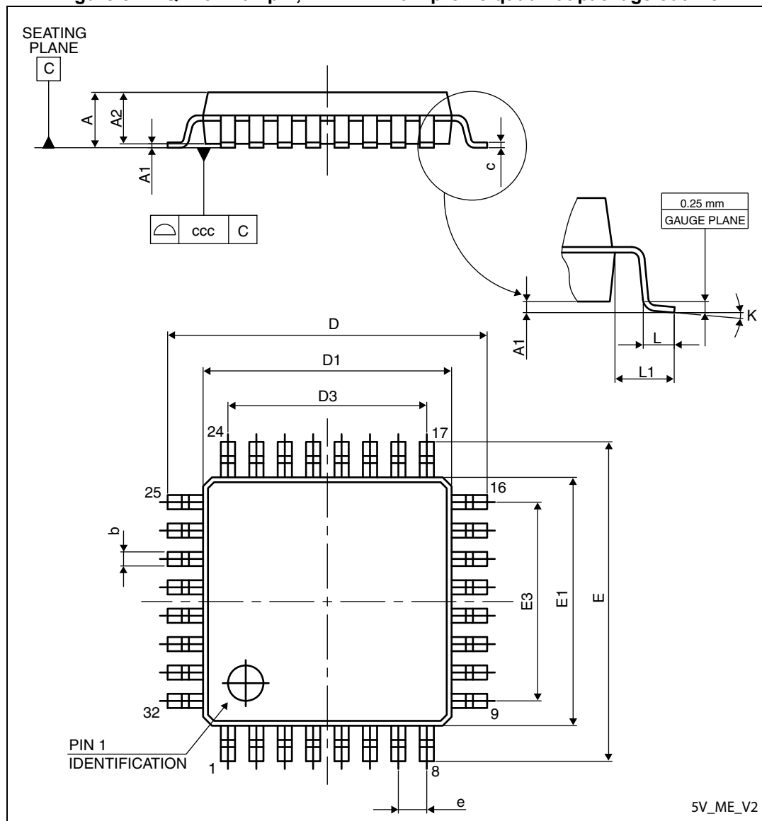
Figure 54. LQFP32 - 32-pin, 7 x 7 mm low-profile quad flat package outline
