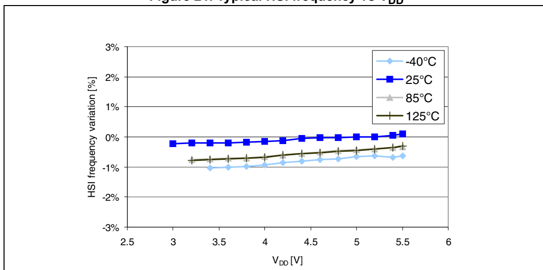
Figure 21. Typical HSI frequency vs V_{DD}
