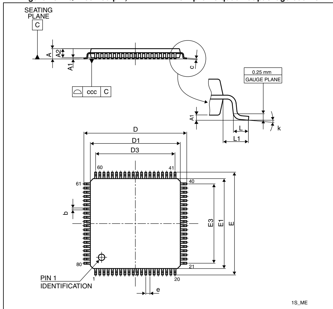
Figure 45. LQFP80 - 80-pin, 14 x 14 mm low-profile quad flat package outline
