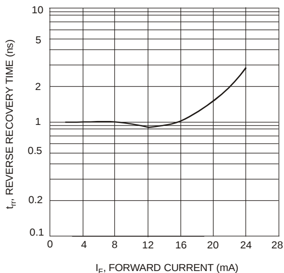
Fig. 4 Typical Reverse Recovery Time Characteristics
