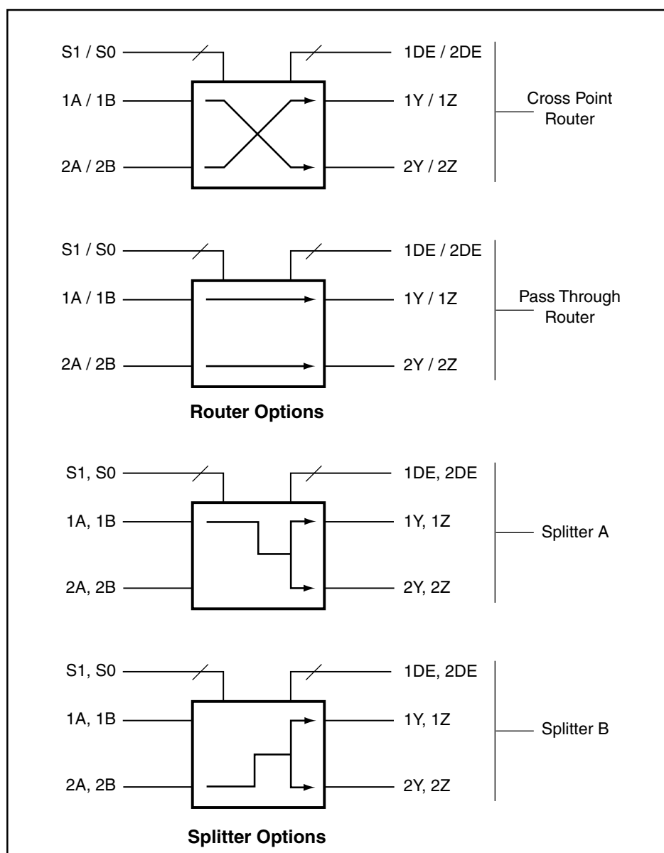
Figure 1. Possible Signal Routing
