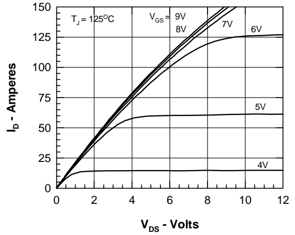
Fig.2 Output Characteristics @ T_j = 125^\circ\text{C}
