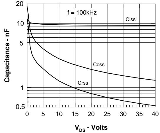
Fig.8 Capacitance Curves
