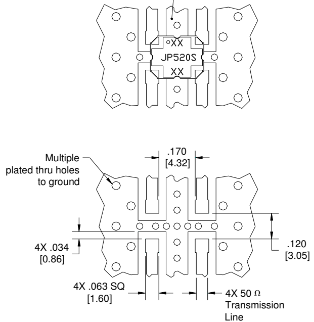
Dimensions are in Inches [Millimeters] JP520S Mounting Footprint
