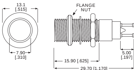
HOLDER WITHOUT COLLAR*
