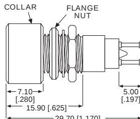
HOLDER WITH COLLAR*
