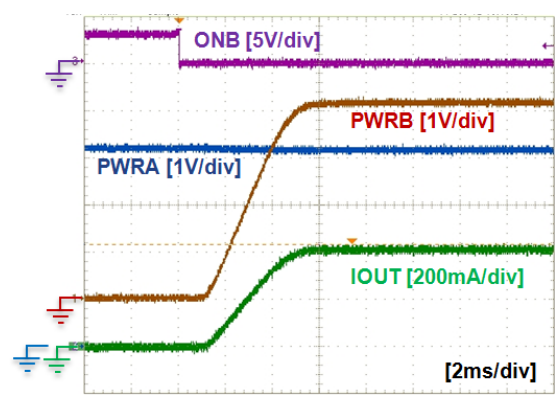
Figure 16. Turn-On Response ( V_{IN}=4.2\text{ V} , C_{IN}=1\ \mu\text{F} , C_{OUT}=1\ \mu\text{F} , R_L=10\ \Omega )
