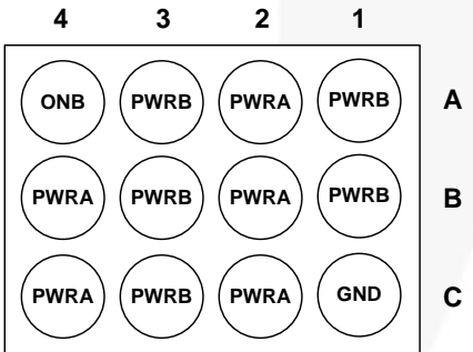
Figure 6. Bottom View
