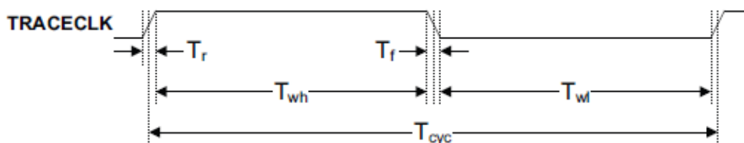
Figure 3. TRACE_CLKOUT specifications
