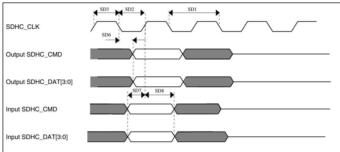
Figure 23. SDHC timing
