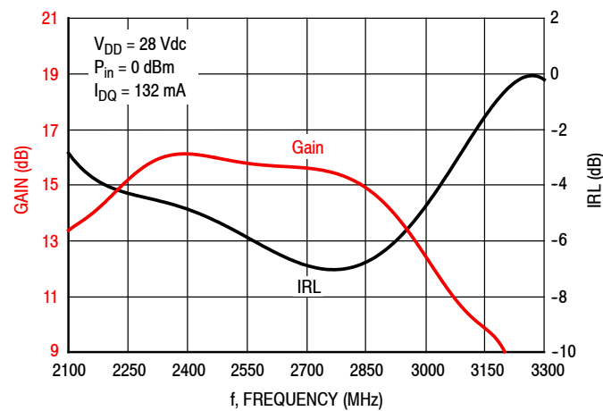
Figure 15. Broadband Frequency Response
