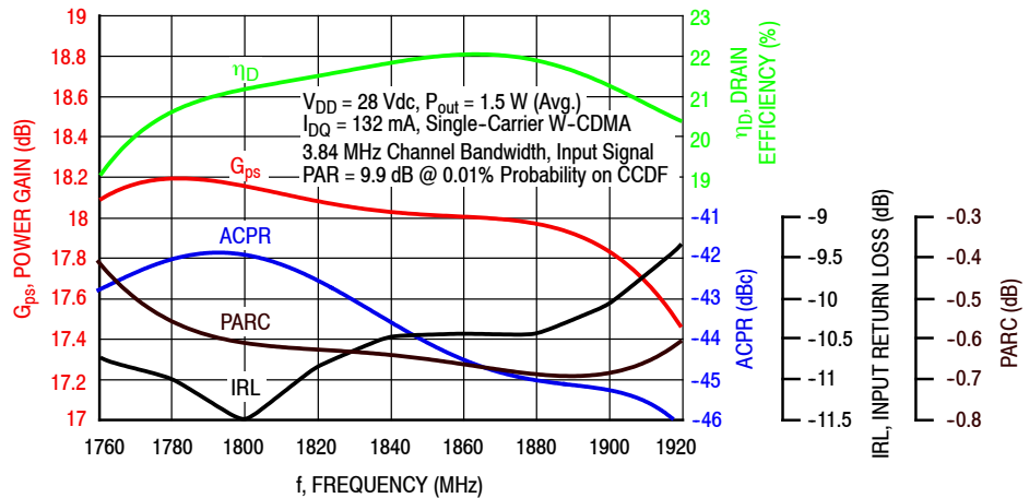
Figure 9. Single-Carrier Output Peak-to-Average Ratio Compression (PARC) Broadband Performance @ P_{out} = 1.5 Watts Avg.
