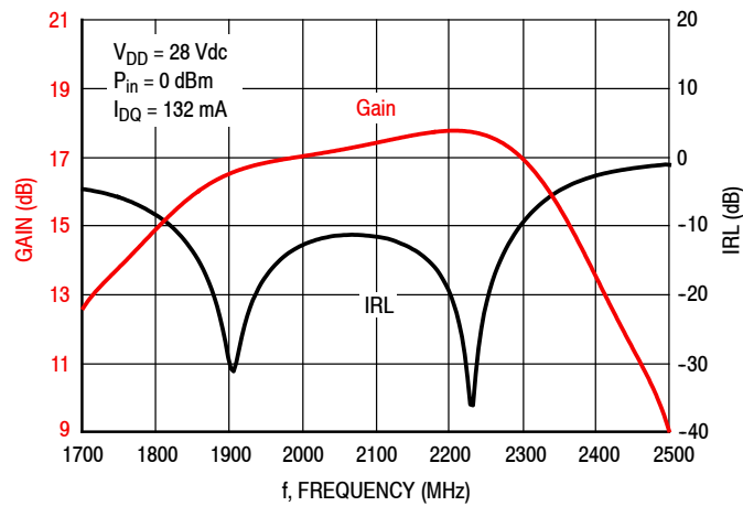
Figure 7. Broadband Frequency Response
