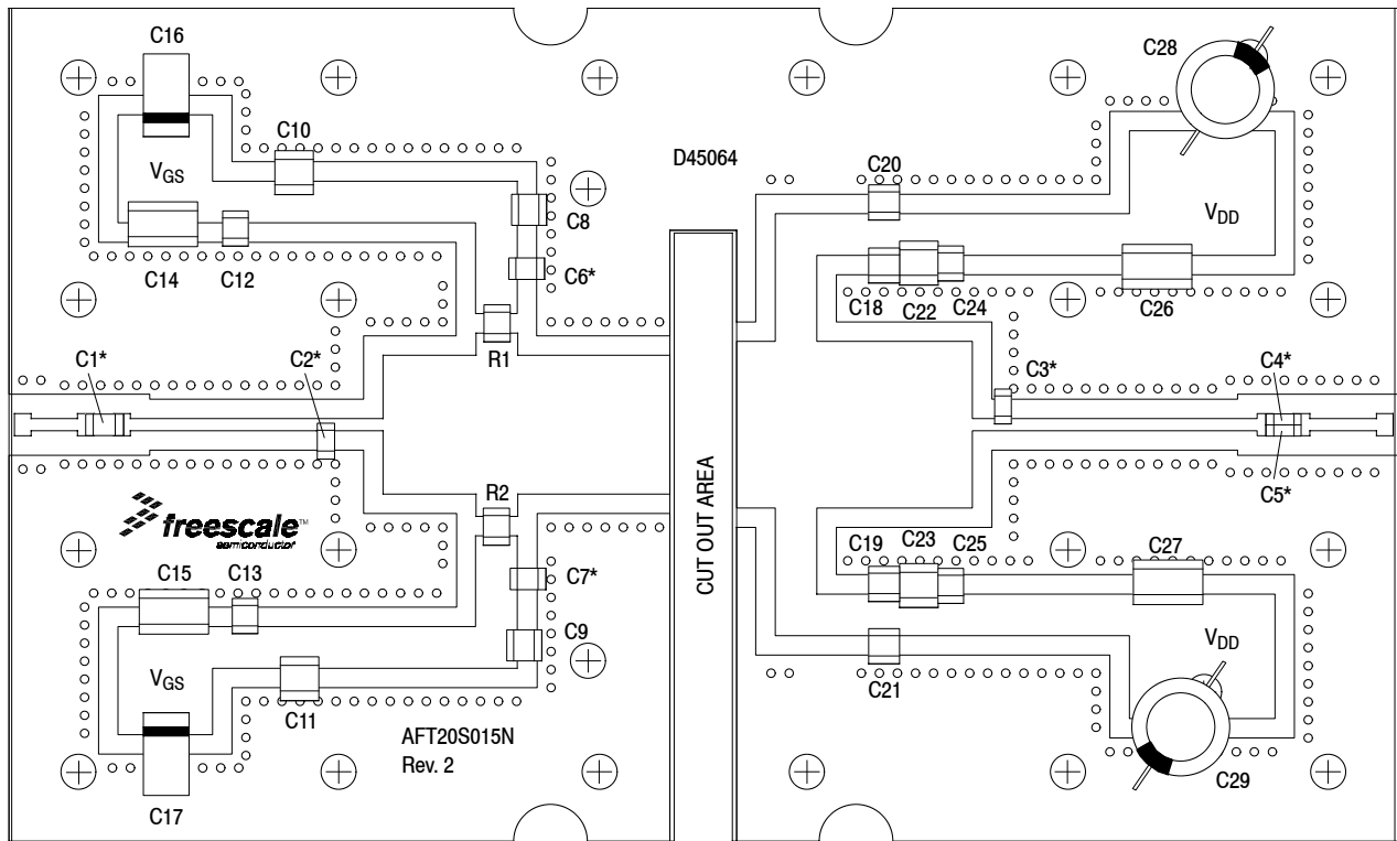
Figure 8. AFT20S015NR1 Test Circuit Component Layout — 1805-1880 MHz
