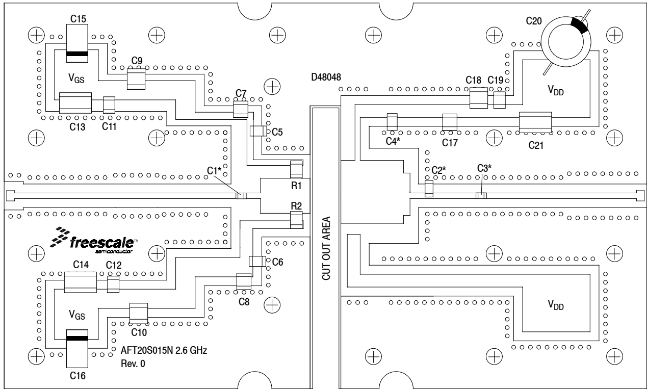
Figure 12. AFT20S015NR1 Test Circuit Component Layout — 2300-2700 MHz
