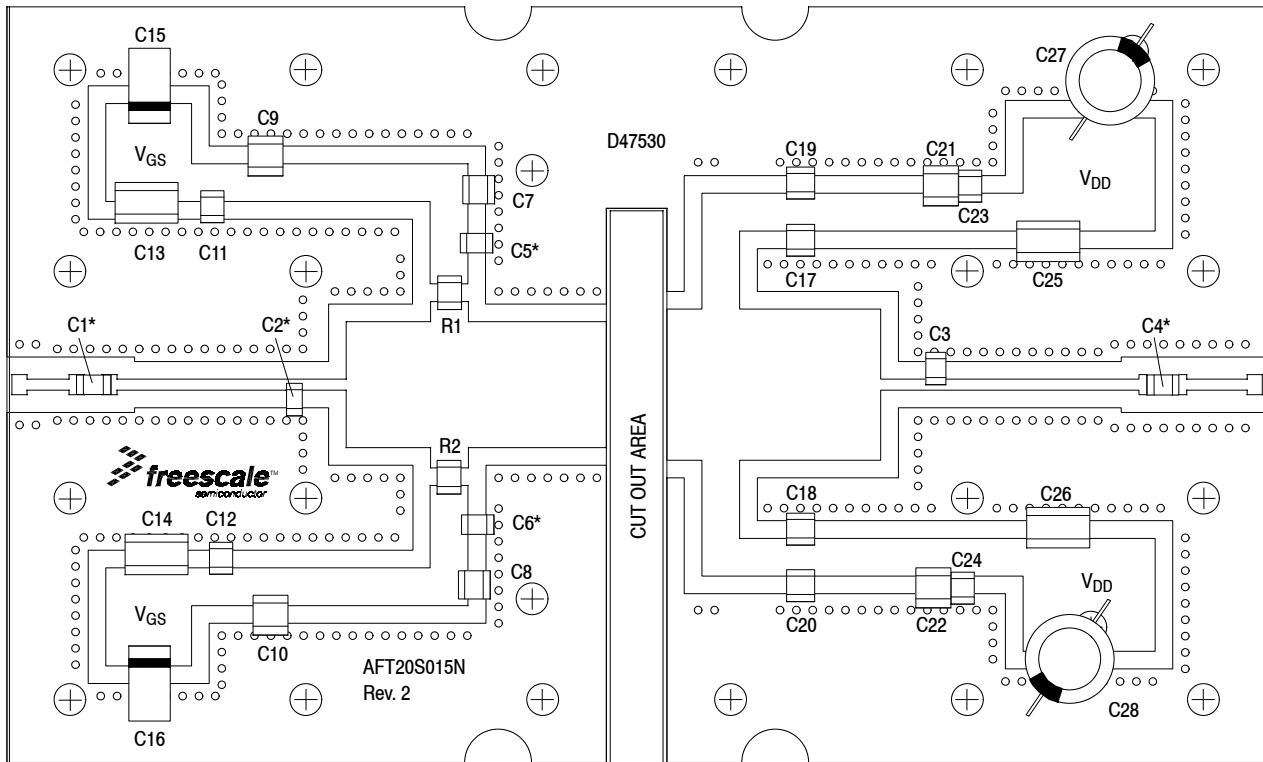
Figure 2. AFT20S015NR1 Test Circuit Component Layout — 2110-2170 MHz
