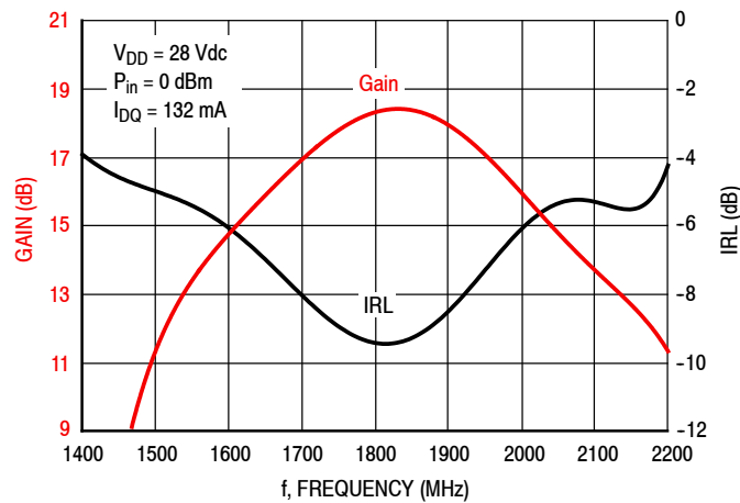
Figure 11. Broadband Frequency Response
