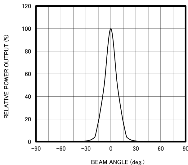
RADIATION PATTERN
