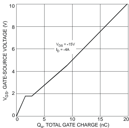
Fig. 10 Gate-Charge Characteristics
