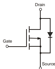
Internal Schematic
