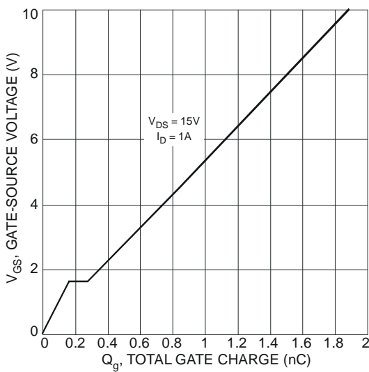
Fig. 11 Gate-Charge Characteristics
