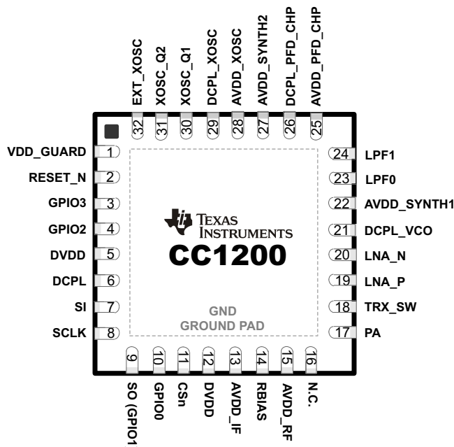
Figure 3-1. Package 5-mm × 5-mm QFN
