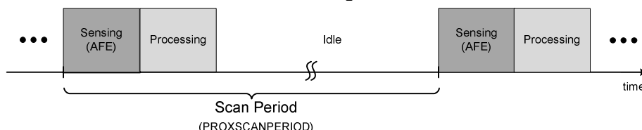
Figure 28 – Proximity Sensing Sequencing
