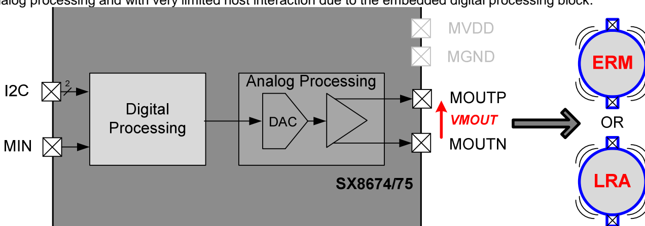
Figure 48 – Haptics Interface Overview
