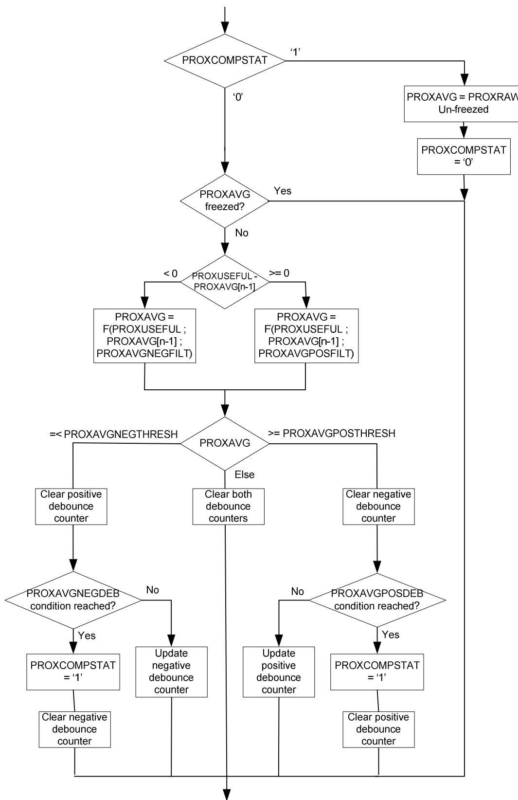
Figure 39 – ProxAvg Update
