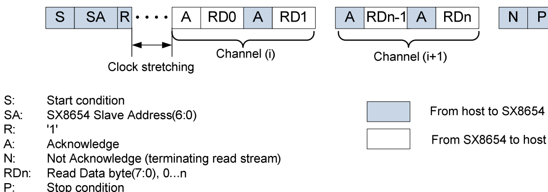
Figure 56 – I2C Read Channel
