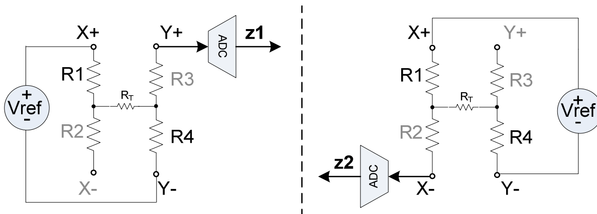
Figure 14 – Pressure Measurement
