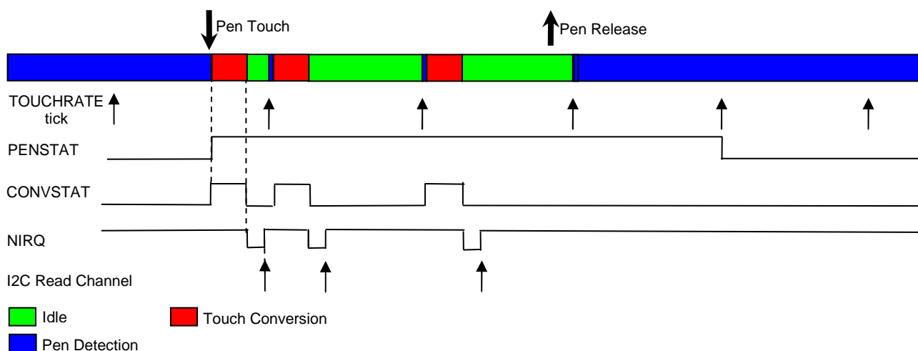
Figure 24 – Pen Trigger Mode ( \text{RegIrqMsk}[3:2] = 10 ; \text{PROXSCANPERIOD} = 0 )
