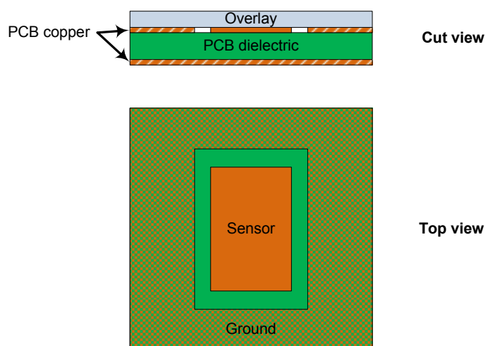
Figure 29 – Typical Capacitive Sensing Implementation
