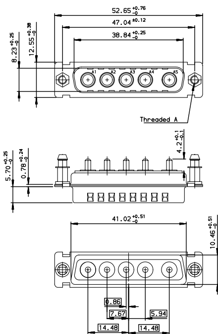
LAYOUT DIMENSIONS (after plating) CONNECTOR SIDE VIEW
