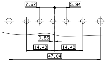
LAYOUT DIMENSIONS (after plating) CONNECTOR SIDE VIEW
