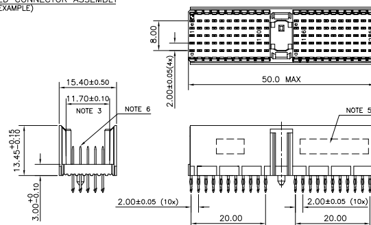
LOADED CONNECTOR ASSEMBLY (FOR EXAMPLE)
