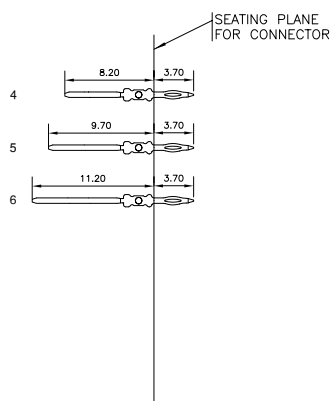
CONTACT OVERVIEW
