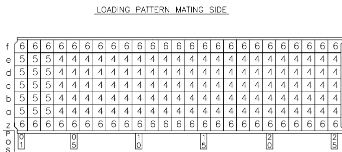
CONTACT OVERVIEW
