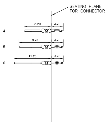
CONTACT OVERVIEW
