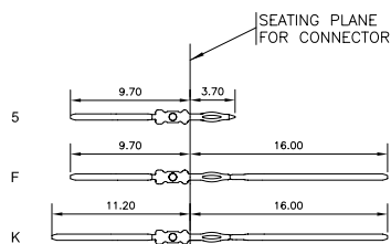
CONTACT OVERVIEW
