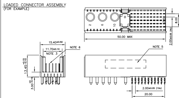
HM2P11PA5110 LEAD FREE INDICATOR : LF ■ LEAD FREE (DIGIT 15 & 16) PLATING CODE (DIGIT 13 AND 14)
