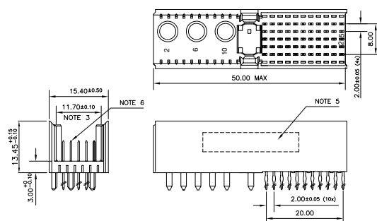
LOADED CONNECTOR ASSEMBLY (FOR EXAMPLE)
