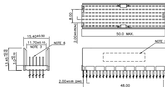
LOADED CONNECTOR ASSEMBLY (FOR EXAMPLE)
