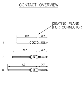
CONTACT OVERVIEW
