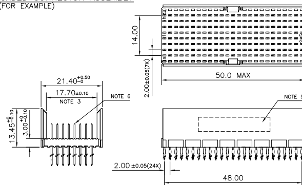
LOADED CONNECTOR ASSEMBLY (FOR EXAMPLE)
