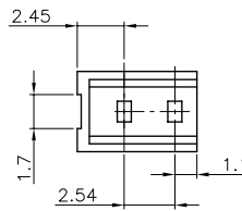
SECTION Z-Z
