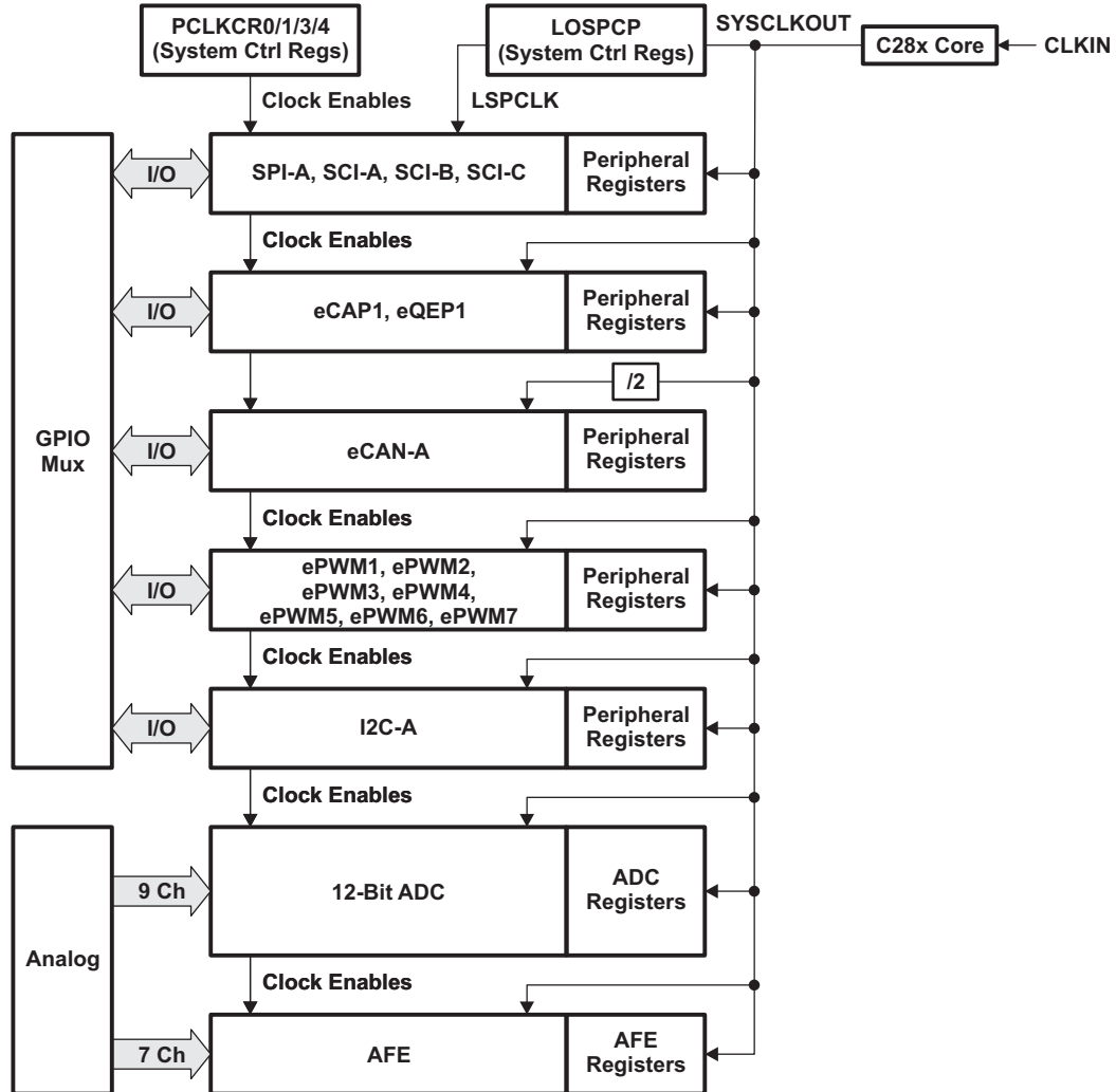
Figure 6-6. Clock and Reset Domains
