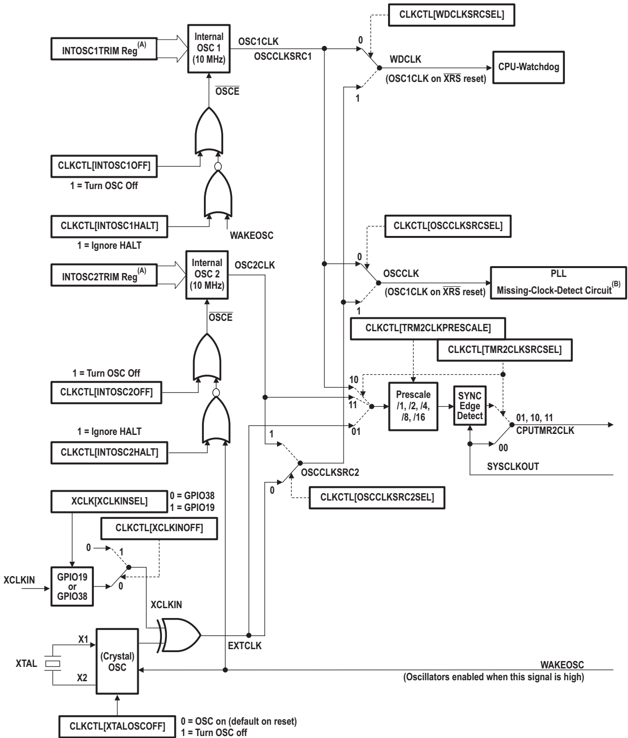
Figure 6-7. Clock Tree
