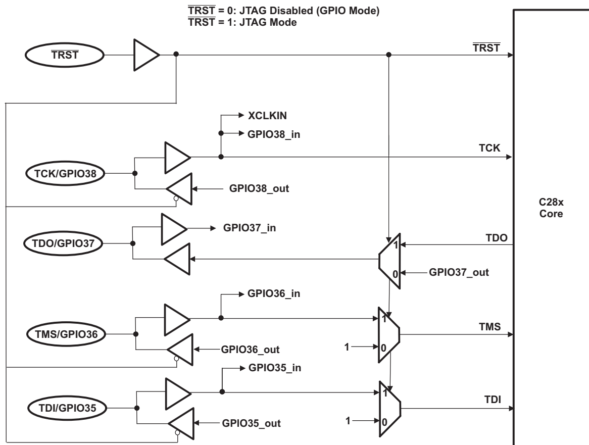
Figure 6-42. JTAG/GPIO Multiplexing
