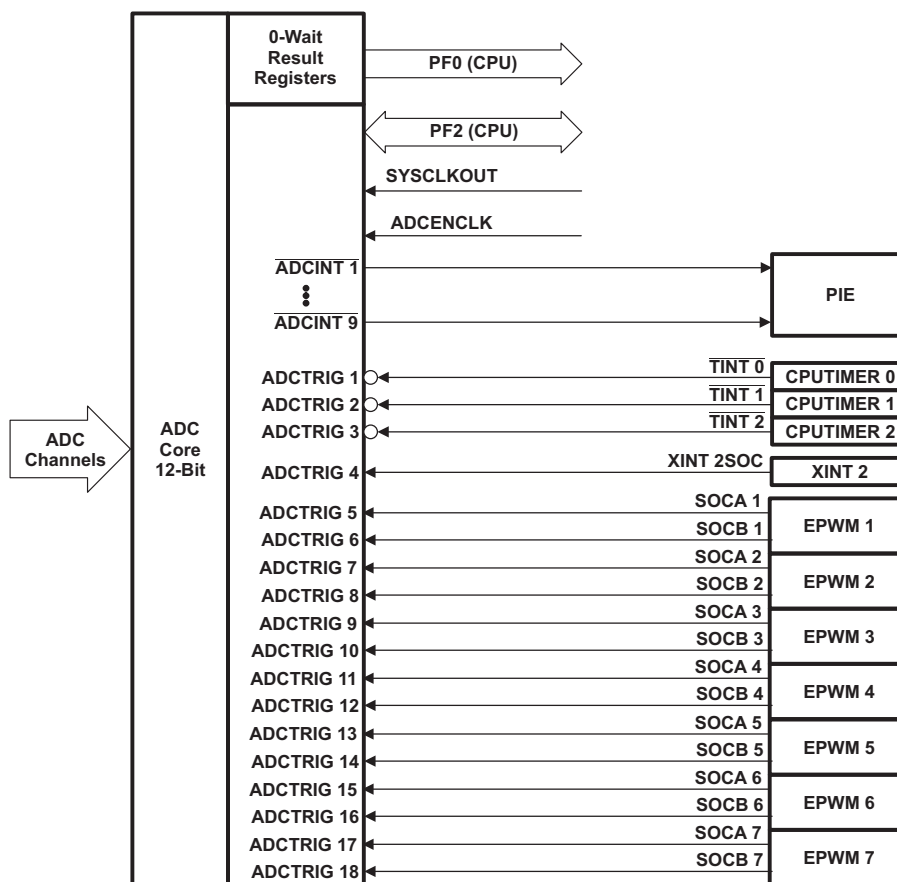
Figure 6-16. ADC Connections
