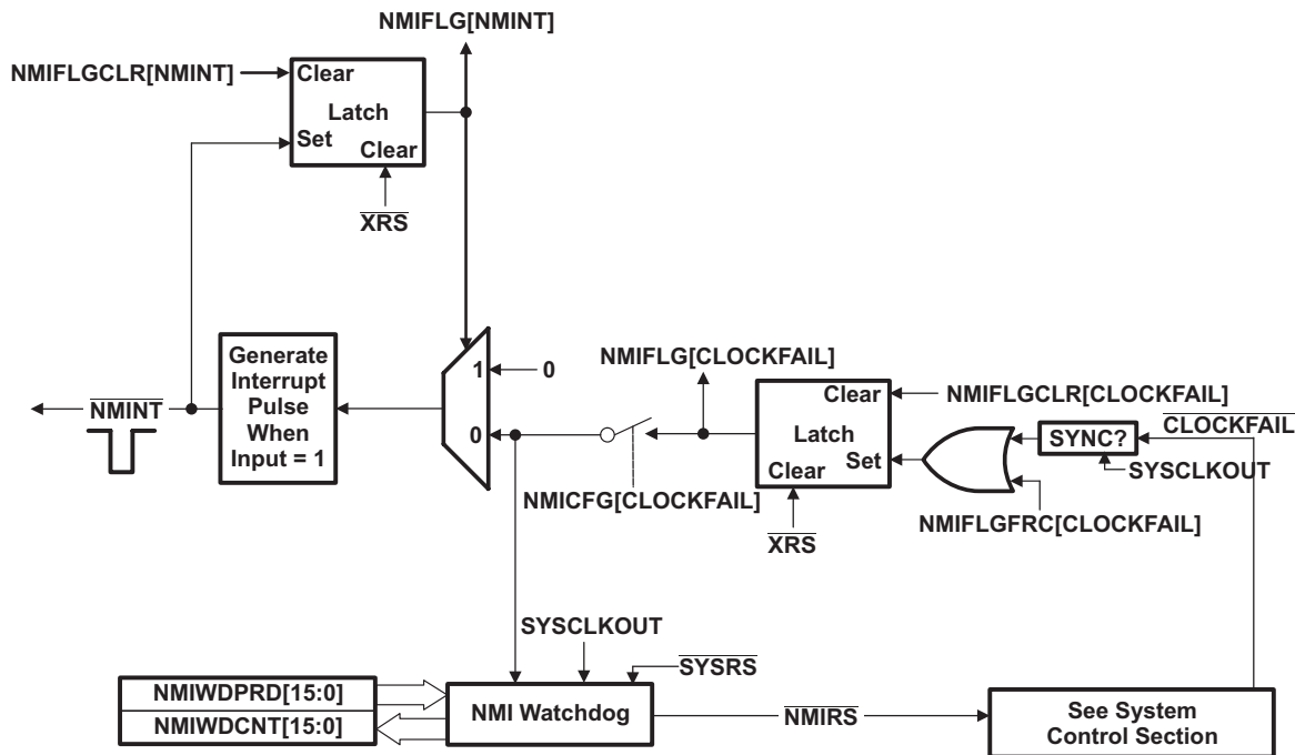
Figure 6-10. NMI-watchdog
