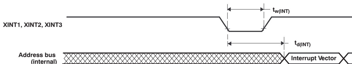
Figure 6-14. External Interrupt Timing
