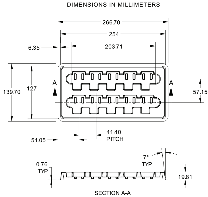
TOP TRAY SHOWN TRANSPARENT FOR REFERENCE ONLY
