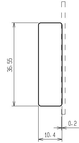
RECOMMENDED PANEL CUT OUT
