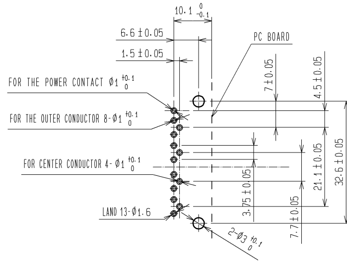
RECOMMENDED PC BOARD HOLE PATTERN
