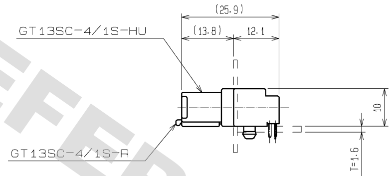
MATED CONNECTORS
