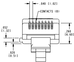
PLUG HOUSING SCALE 2.5
