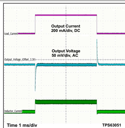
Figure 29. Load Transient Response
