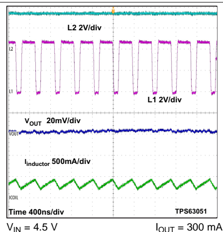
Figure 27. Switching Waveform in Buck Mode and PWM
