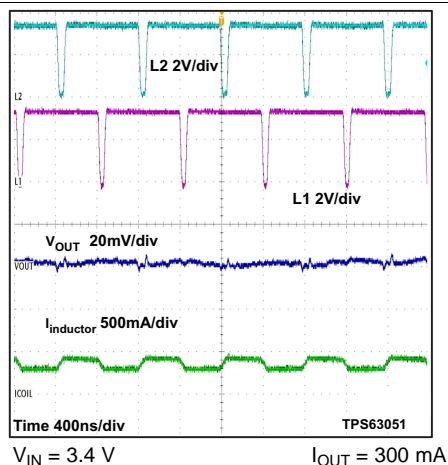
Figure 28. Switching Waveform in Buck-Boost Mode and PWM
