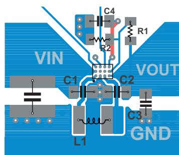
Figure 34. TPS6305x Layout (WCSP)
