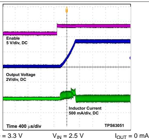
Figure 32. Start Up After Enable
