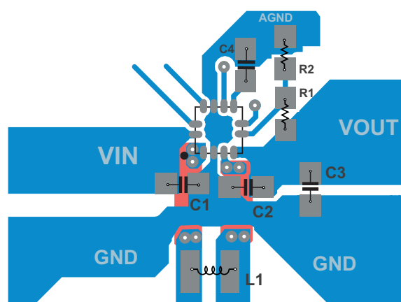
Figure 35. TPS6305x Layout (HotRod)
