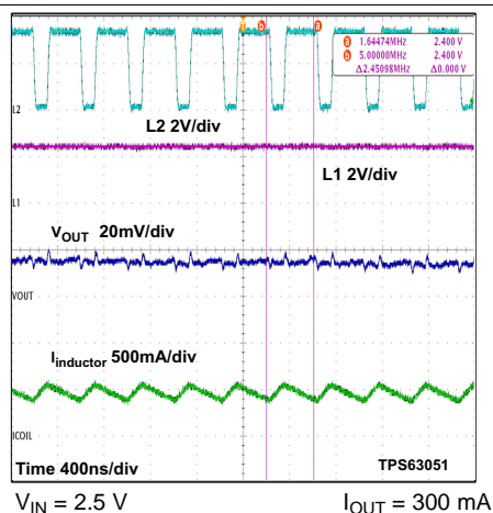
Figure 26. Switching Waveform in Boost Mode and PWM
