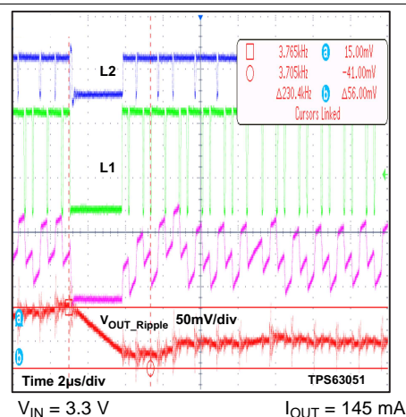
Figure 23. Output Voltage ripple in Buck-Boost mode and PFM to PWM transition
