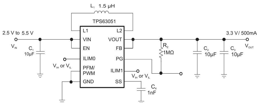
Figure 8. Parameter Measurement Circuit (WCSP)
