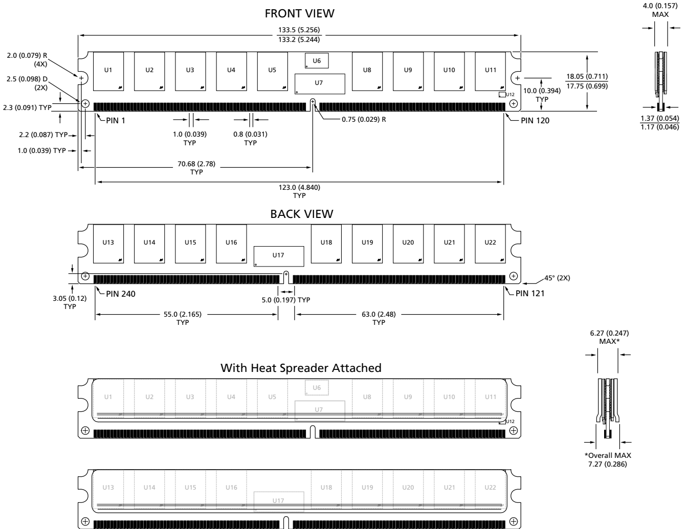
Figure 3: 240-Pin DDR2 VLP RDIMM
