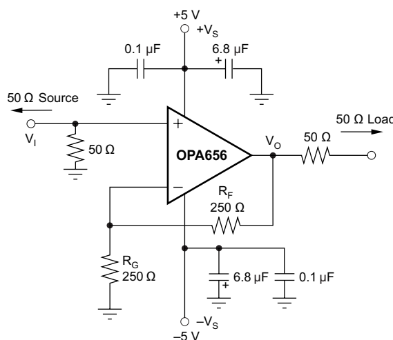
Figure 29. Noninverting G = +2 V/V Specifications and Test Circuit
