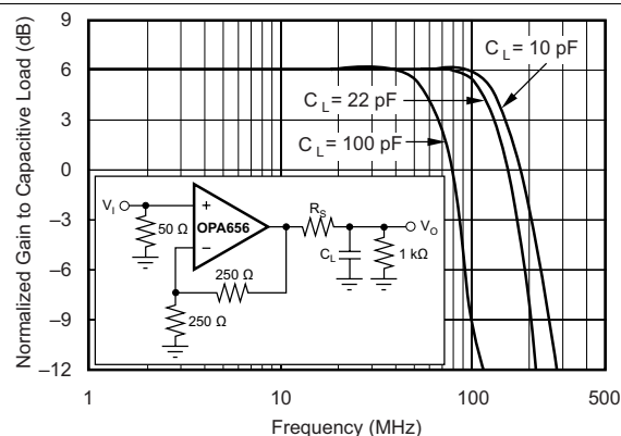
Figure 18. Frequency Response vs Capacitive Load
