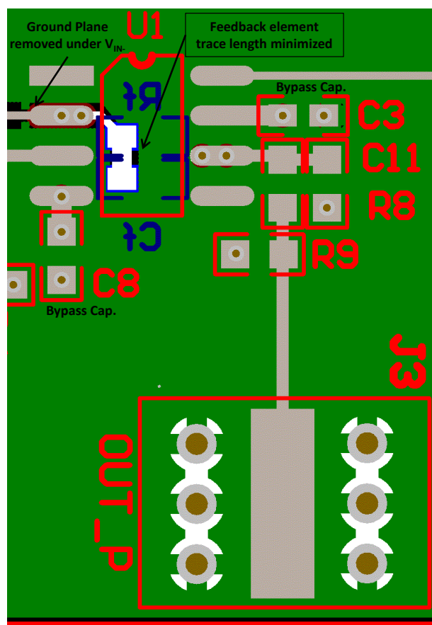
Figure 35. Layout Recommendation
