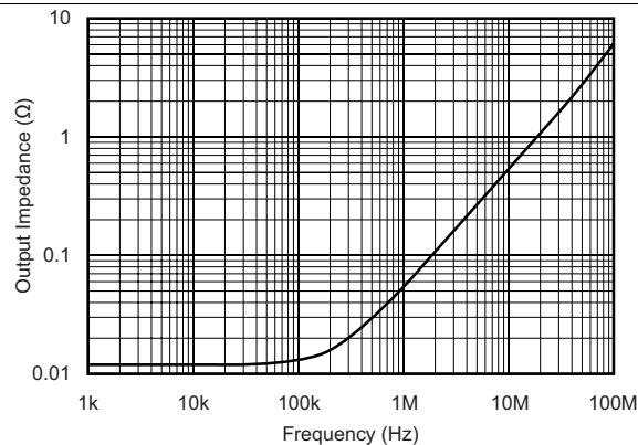
Figure 26. Closed-Loop Output Impedance vs Frequency
