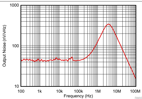
Figure 33. Measured Total TIA Noise
