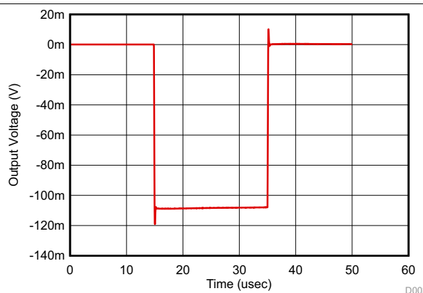
Figure 34. Transient Pulse Response to 2-μA Input Current Pulse
