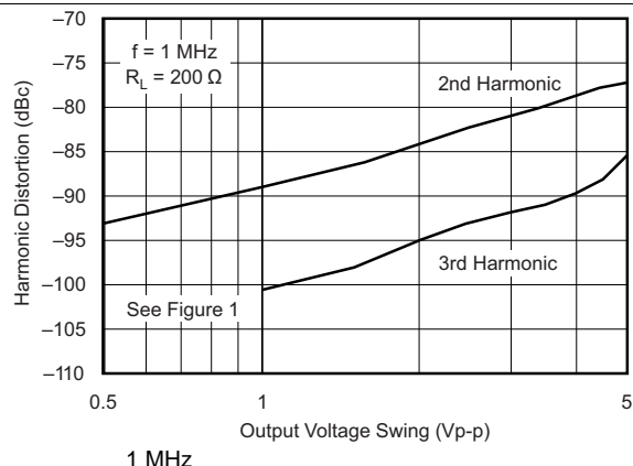
Figure 10. Harmonic Distortion vs Output Voltage
