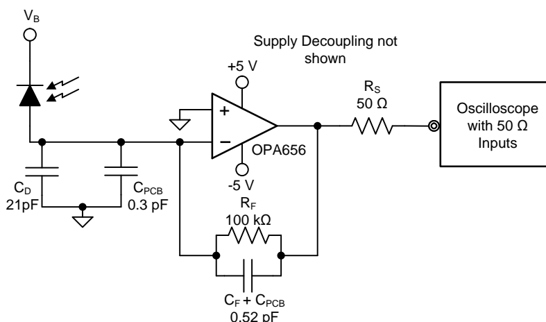
Figure 32. Wideband, High-Sensitivity, Transimpedance Amplifier
