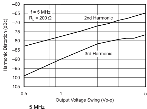
Figure 8. Harmonic Distortion vs Output Voltage
