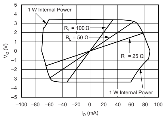
Figure 25. Output Voltage and Current Limitations
