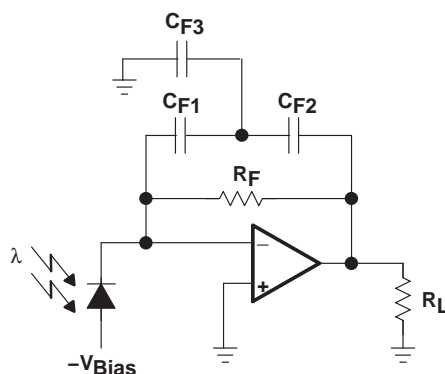
Figure 35. Alternative Transimpedance Configuration #3
