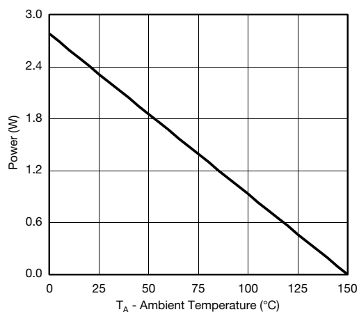
Power, Junction-to-Ambient
