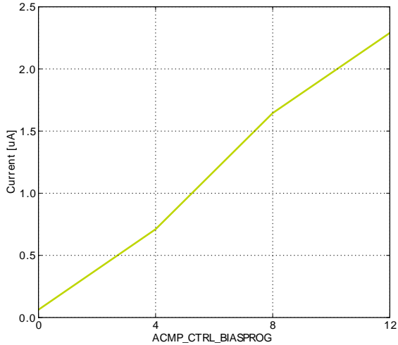
Current consumption, HYSTSEL = 4
