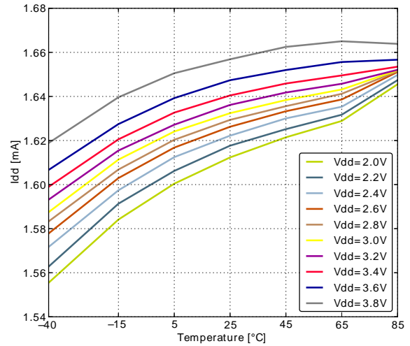
Figure 3.4. EM0 Current consumption while executing prime number calculation code from flash with HFRCO running at 11 MHz
