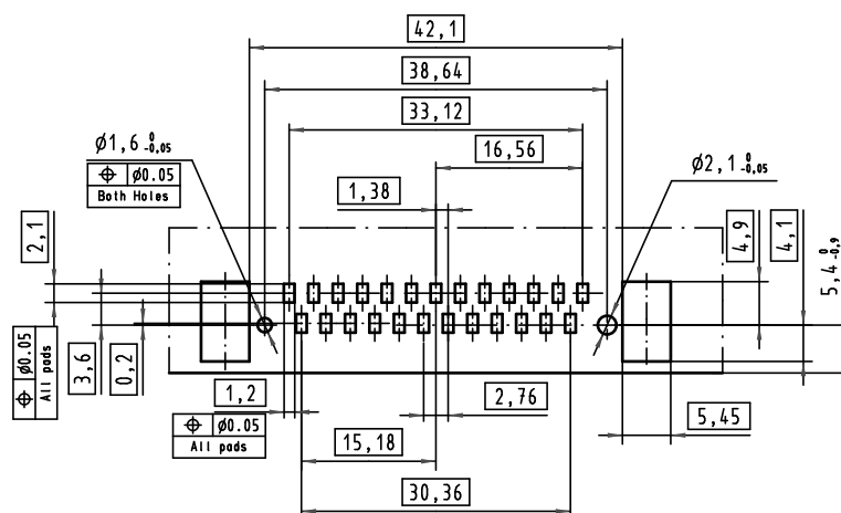
PCB Layout, component side (thickness 1,6mm min.)
