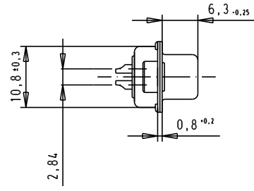
Solder bucket for AWG 20 Max
