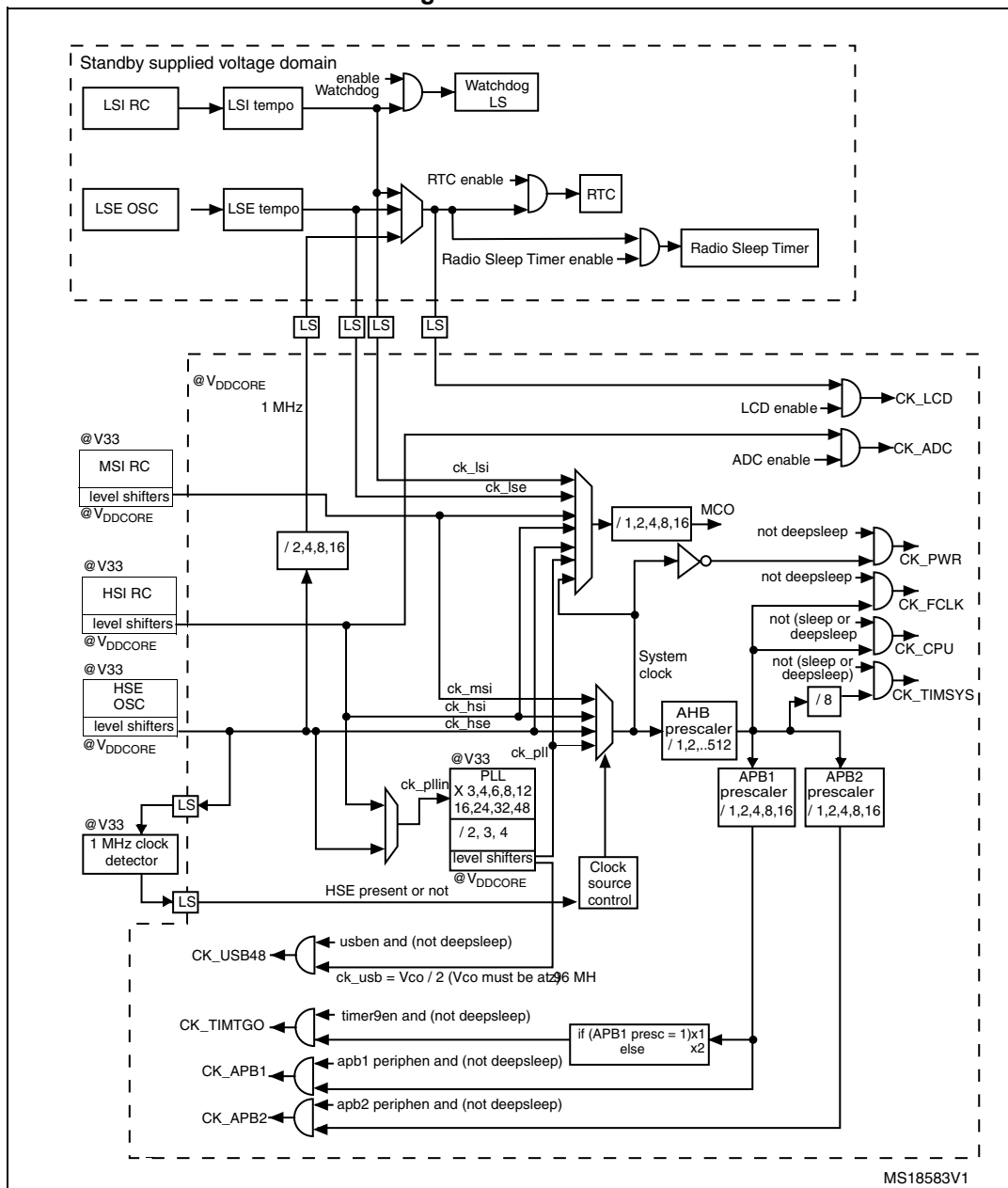
Figure 2. Clock tree
