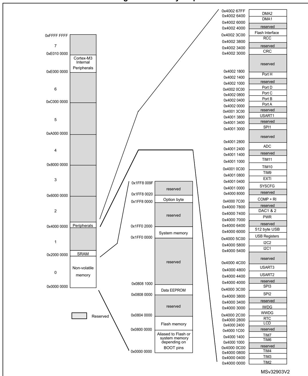
Figure 4. Memory map
