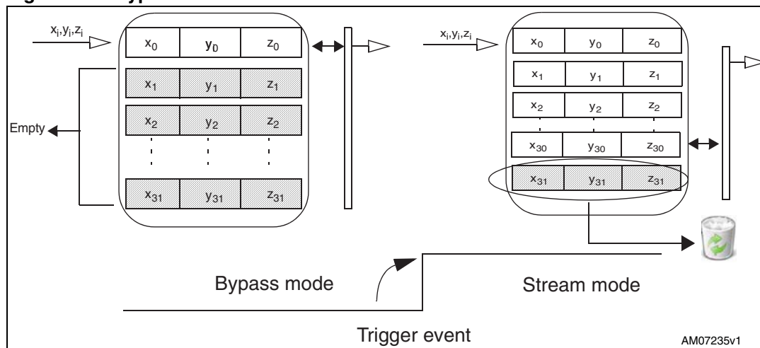
Figure 10. Bypass-to-stream mode
