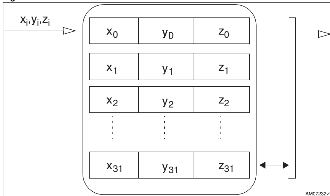
Figure 8. FIFO mode
