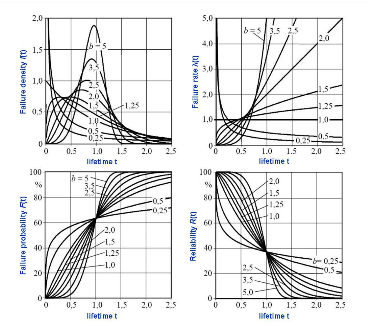
Figure 12: Weibull distribution for various shape parameters b and with a characteristic lifetime of T = 1
