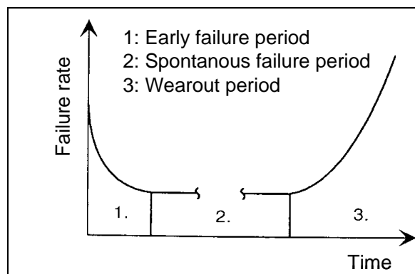
Figure 2: Failure rate over time ("bathtub curve")
