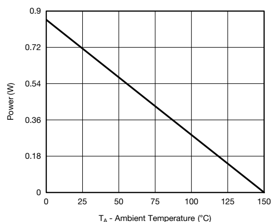
Power Junction-to-Ambient
