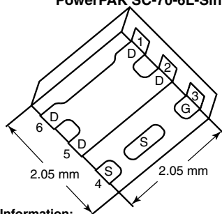
PowerPAK SC-70-6L-Single
