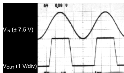
Figure 46. A \pm 7.5\text{ V} Input Signal Greatly Exceeds the 3-V Supply in Figure 47 Causing No Phase Inversion Due to R_I
