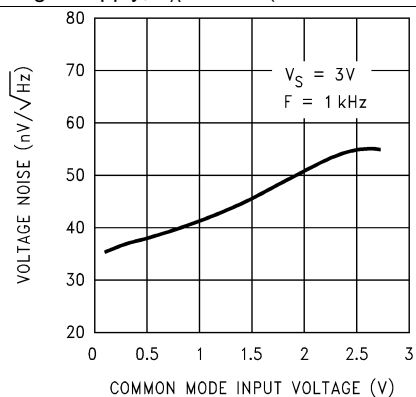
Figure 13. Input Voltage Noise vs Input Voltage
