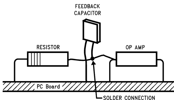
Figure 77. Air Wiring
