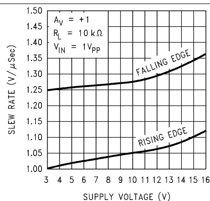
Figure 63. Slew Rate vs Supply Voltage
