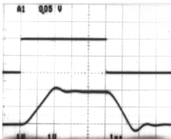
Figure 52. Pulse Response of LMC6484 Circuit in Figure 51
