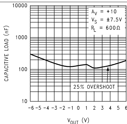
Figure 44. Stability vs Capacitive Load
