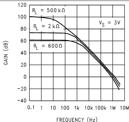
Figure 56. Open Loop Frequency Response
