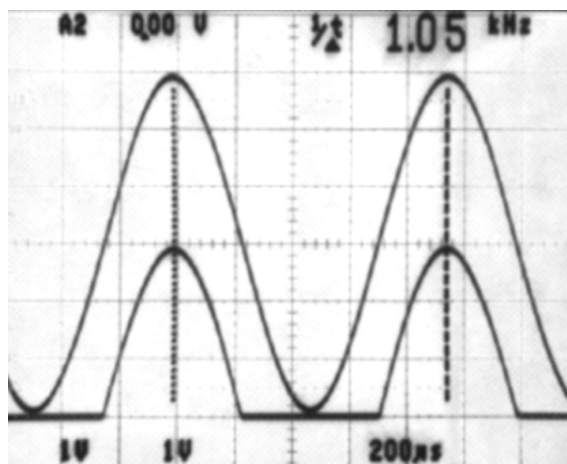
Figure 65. Half-Wave Rectifier Waveform
