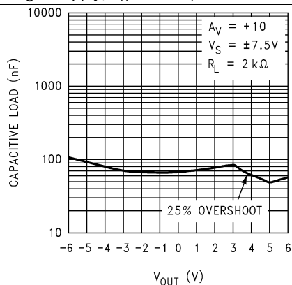
Figure 43. Stability vs Capacitive Load
