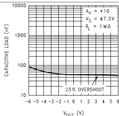
Figure 40. Stability vs Capacitive Load
