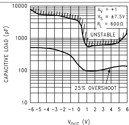
Figure 39. Stability vs Capacitive Load
