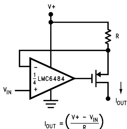
Figure 68. Large Compliance Range Current Source
