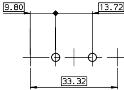
LAYOUT DIMENSIONS (after plating) CONNECTOR SIDE VIEW
